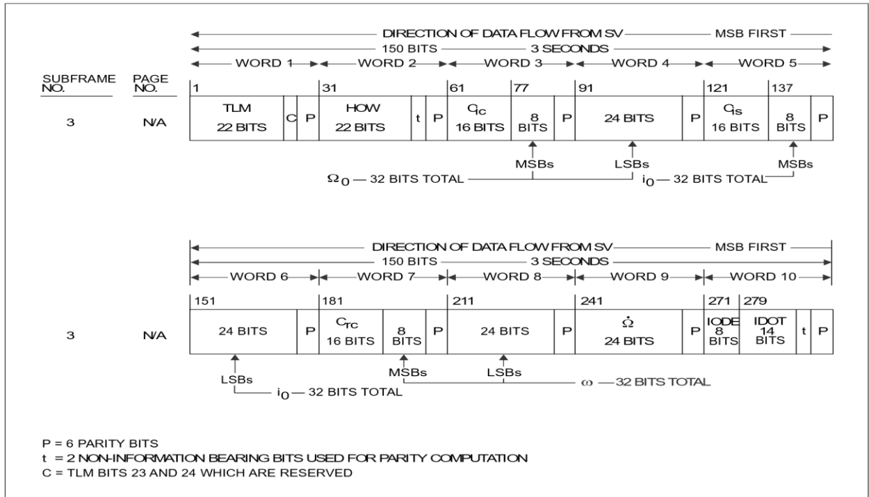
Figure B-6. Data format (3 of 11)
