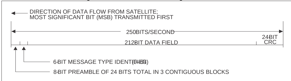
Figure B-11. Convolutional encoding
