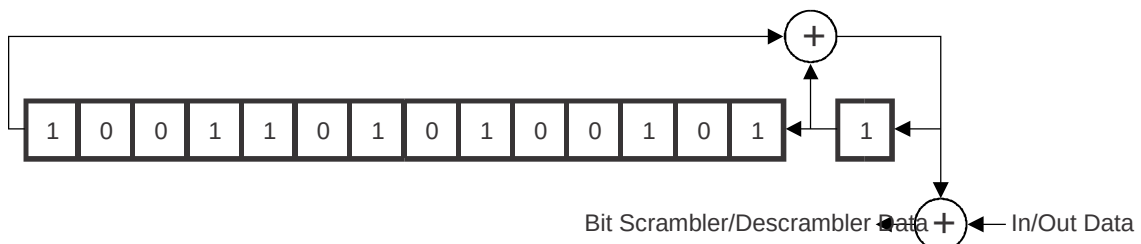
Figure D-6. Bit scrambler/descrambler
