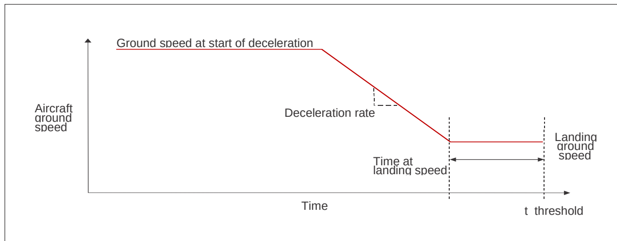
Figure D-8. Aircraft speed profile model
