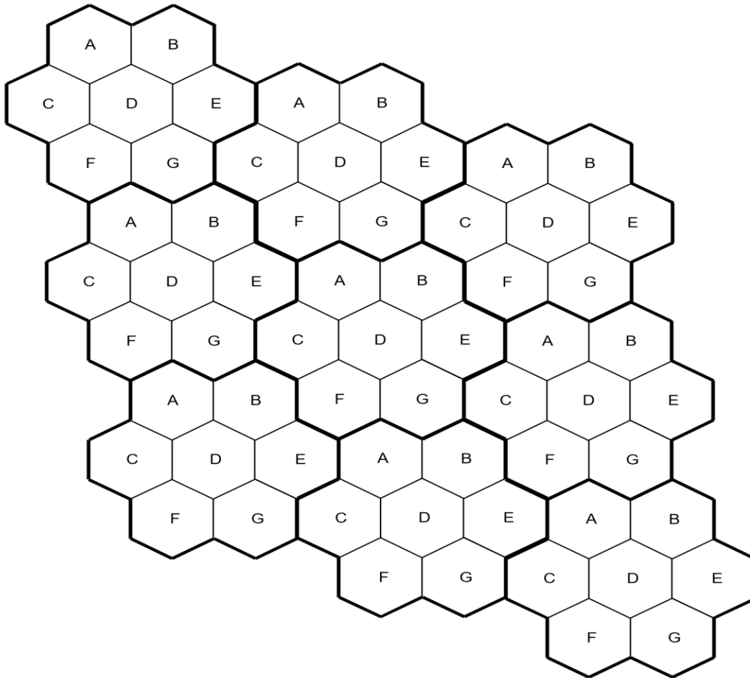
Figure D-5A. Single frequency GRAS VHF networking using multiple time slots
