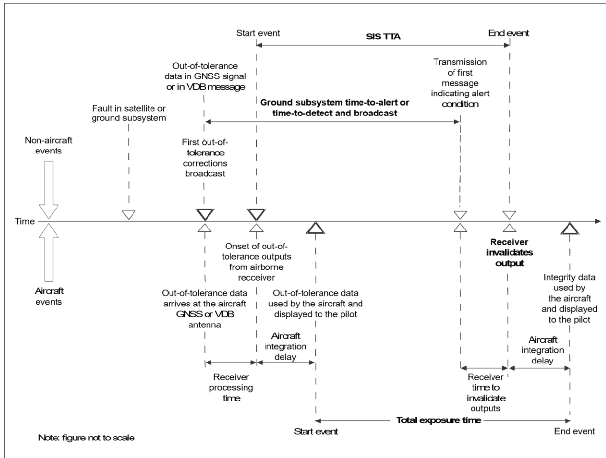
Figure D-13. Nominal GBAS time-to-alert illustration
