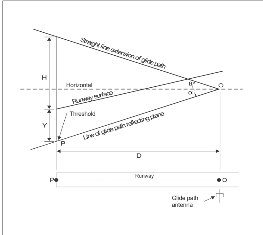
Figure C-5. Glide path siting for sloping runway
