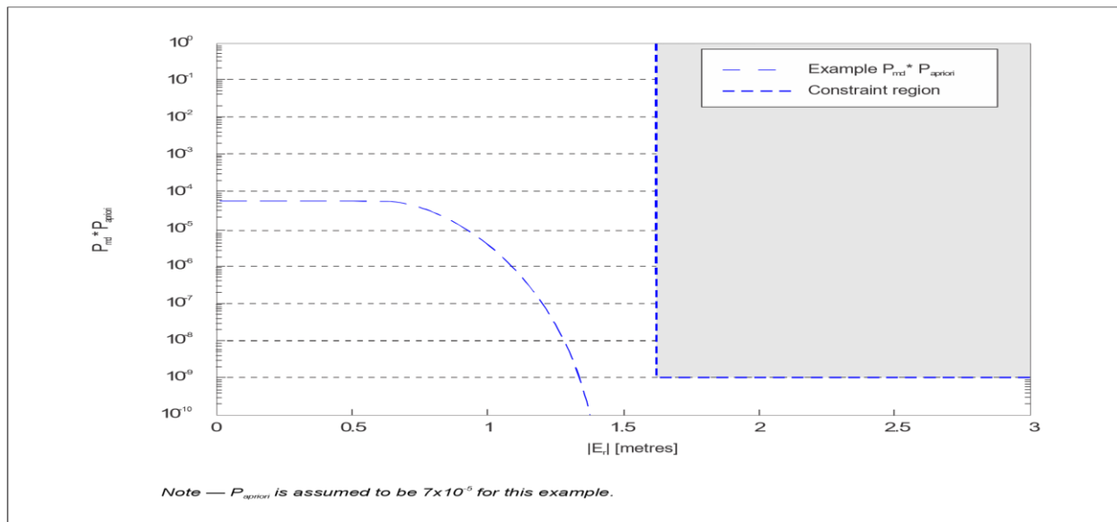
Figure D-12. Example P_{md\_limit} constraint with a priori probability
