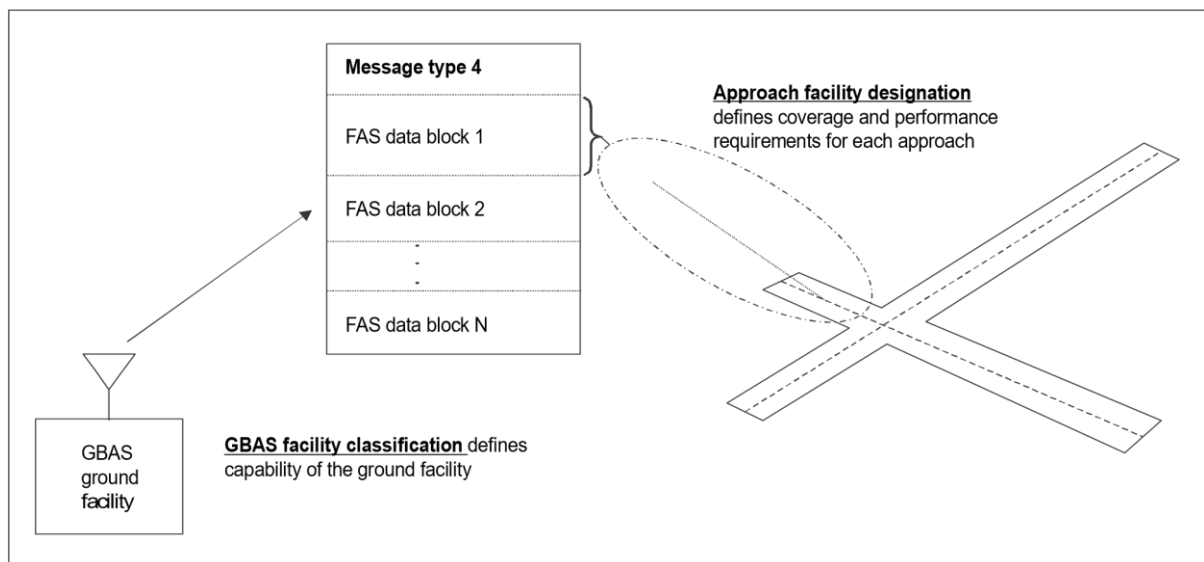
Figure D-4 Relationship between GBAS facility classification and approach facility designation
