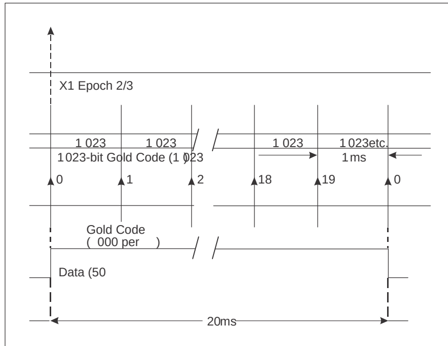
Figure B-1. C/A code timing relationships
