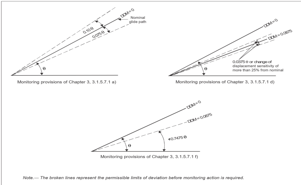
Figure C-12. Glide path monitoring provisions
