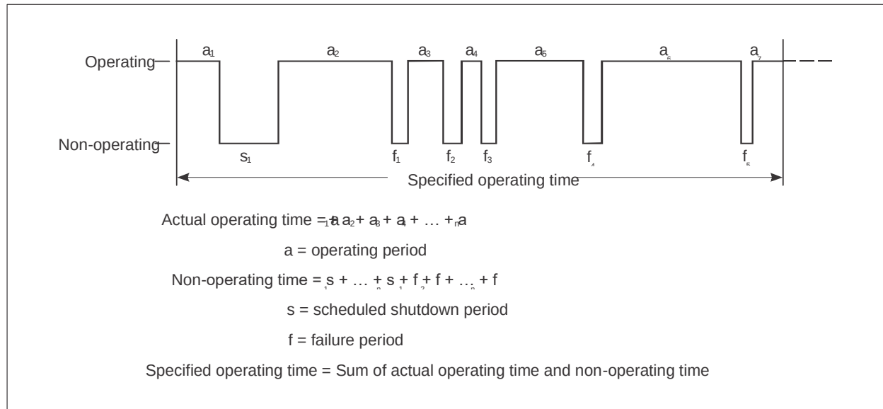
Figure F-2. Evaluation of facility availability and reliability
