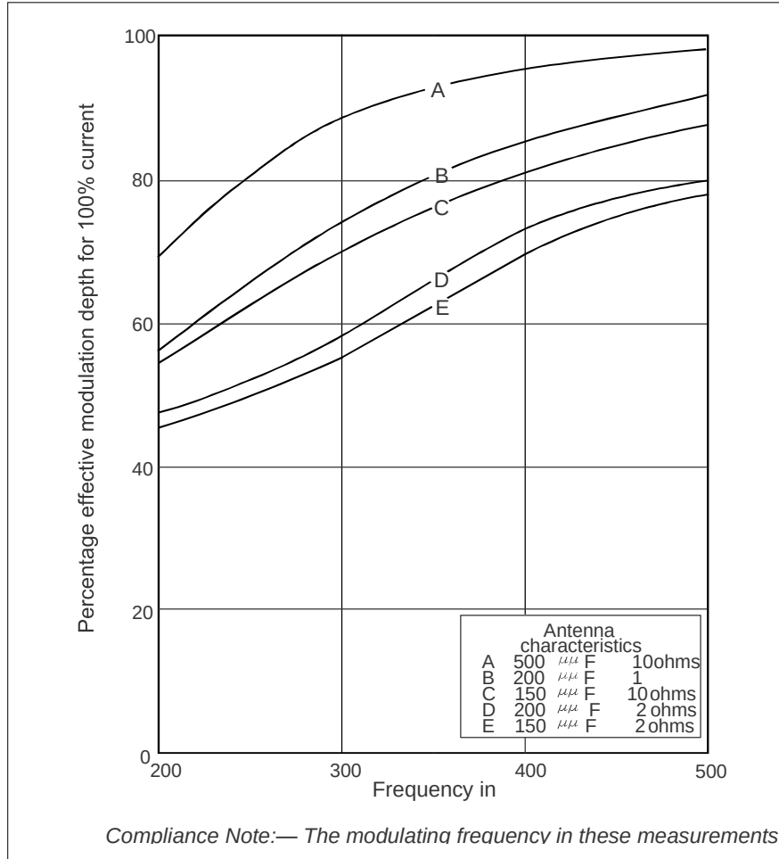
Figure C-19. The effect of antenna Q on the depth of modulation of the radiated signal
