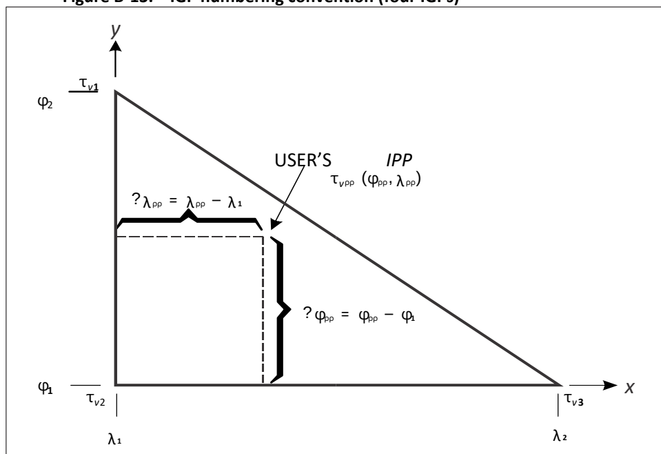
Figure B-13. IGP numbering convention (four IGPs)
