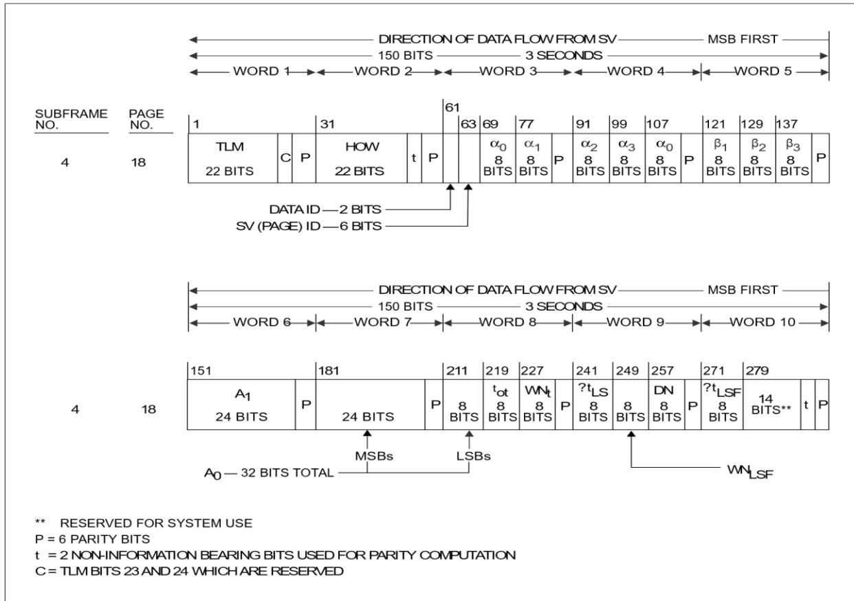
Figure B-6. Data format (8 of 11)
