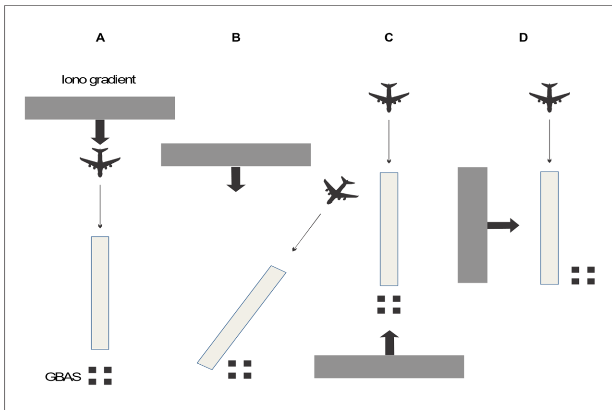
Figure D-10. Ionospheric gradient air/ground/approach orientations
