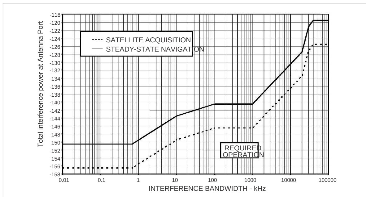
Figure B-17. Interference thresholds versus bandwidth for GPS and SBAS receivers
