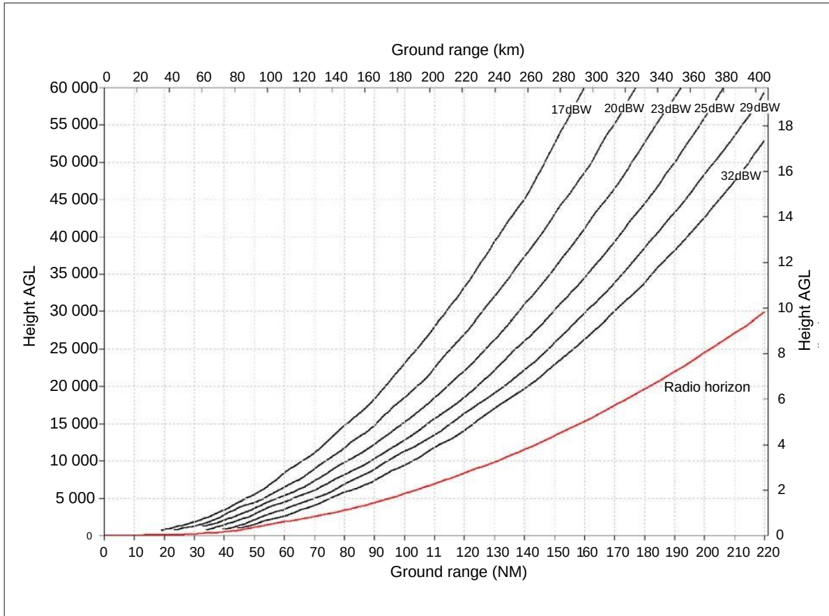
Figure C-13. Necessary EIRP to achieve a field strength of 90 microvolts per metre ( -107 \text{ dBW/m}^2 ) as a function of height above and distance from the VOR/DVOR
