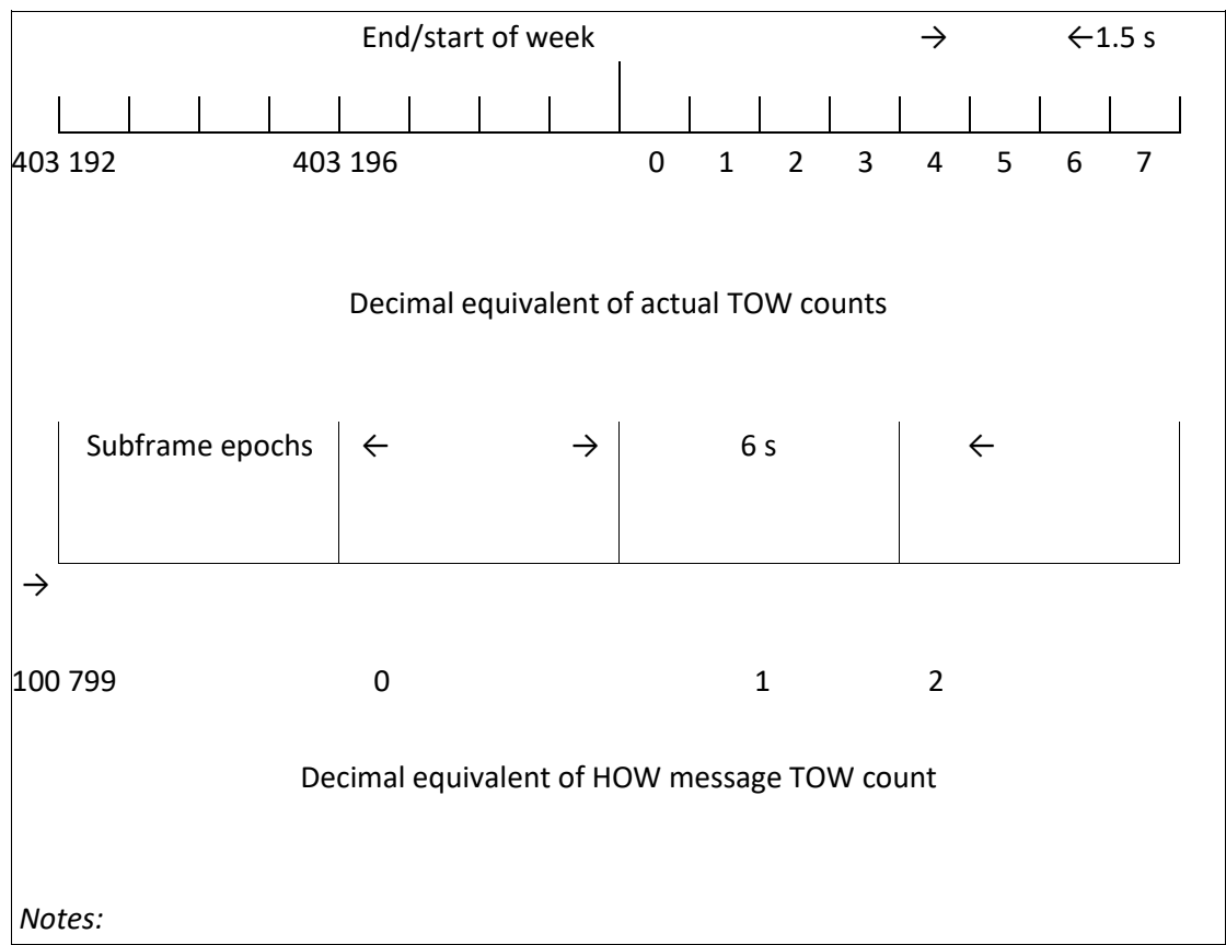
Figure B-4. HOW format
