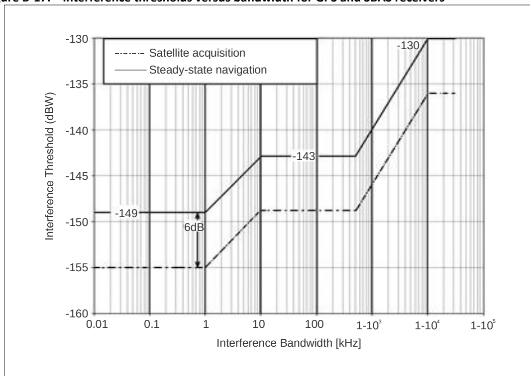
Figure B-17. Interference thresholds versus bandwidth for GPS and SBAS receivers
