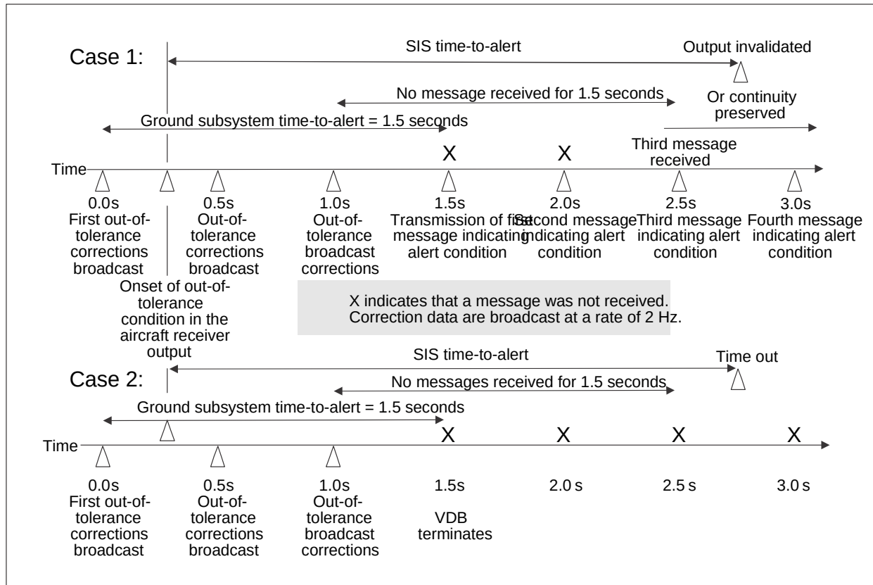
Figure D-14. Effect of missed messages on the GAST D GBAS time-to-alert below 200 ft Case 1 describes the situation for missed messages, Case 2 the one for VDB termination
