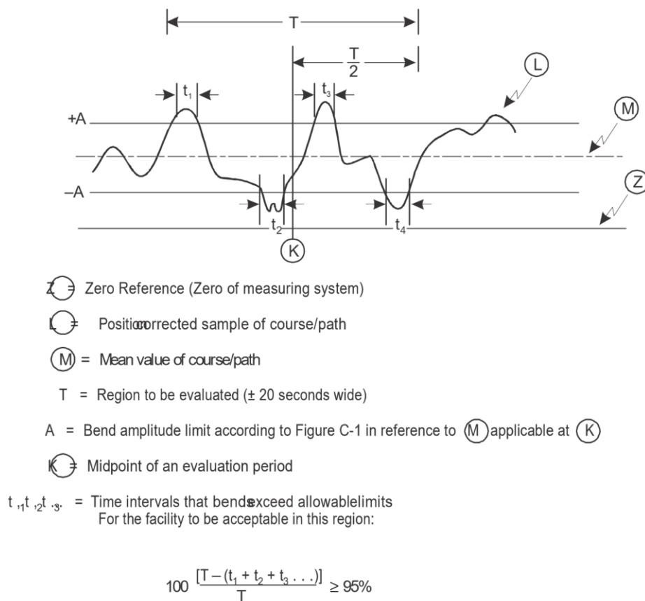
Figure C-2. Evaluation of course/path bend amplitude
