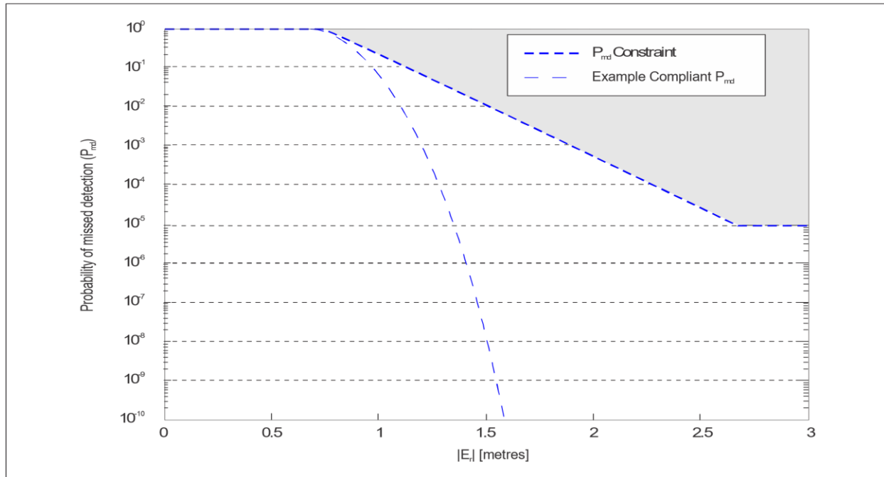
Figure D-11. Example P_{md\_limit} constraint region
