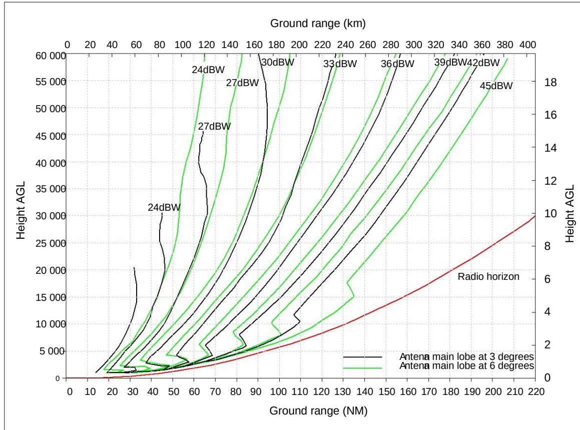
Figure C-20. Necessary EIRP to achieve a power density of -89 \text{ dBW/m}^2 as a function of height above and distance from the DME
