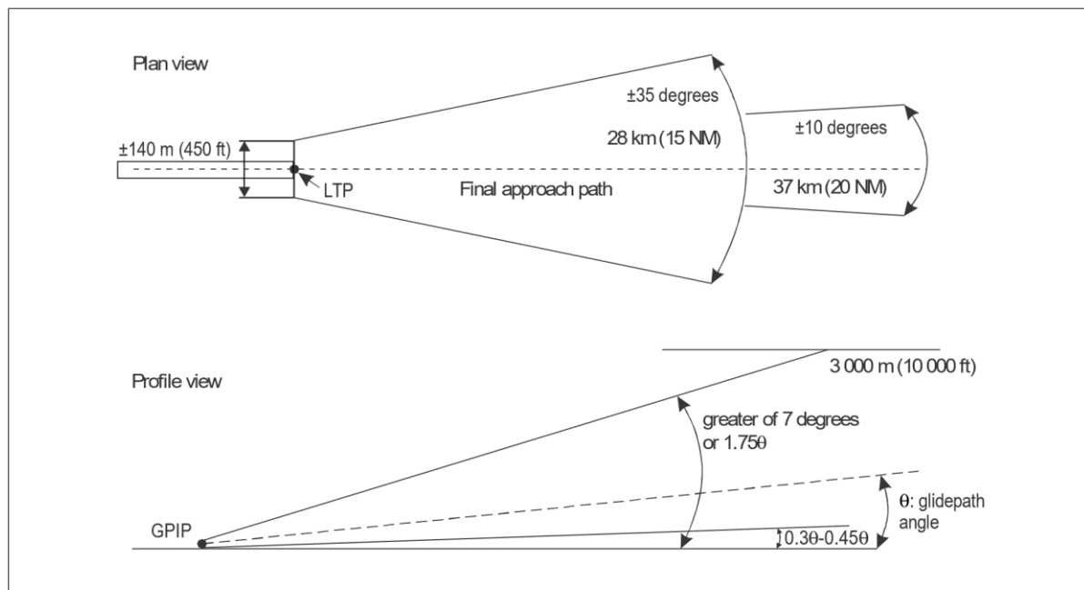
Figure D-5. Minimum GBAS service volume
