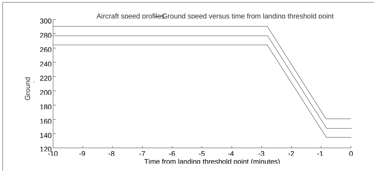
Figure D-9. Family of aircraft speed profiles
