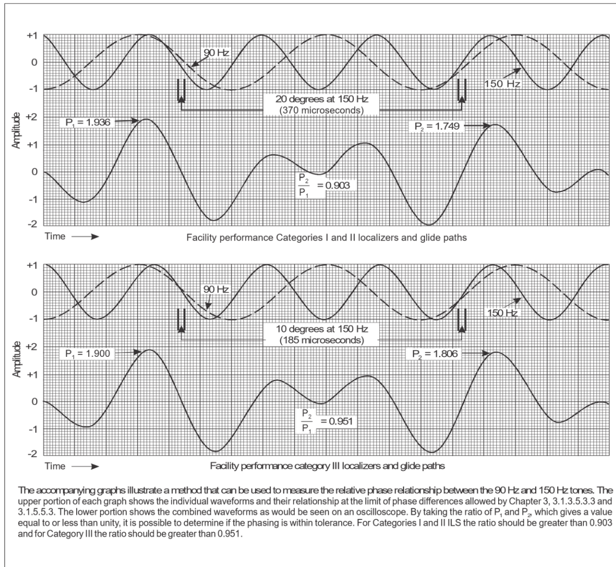
Figure C-6. ILS wave forms illustrating relative audio phasing of the 90 Hz and 150 Hz tones
