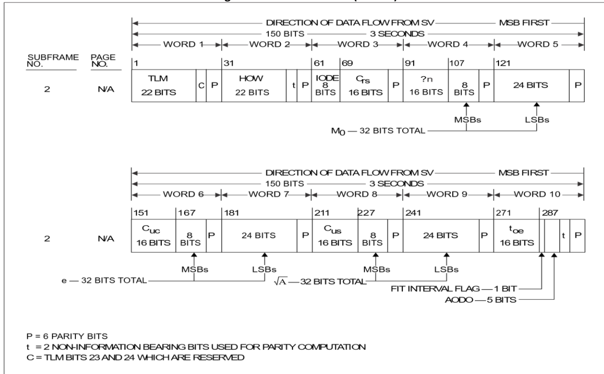
Figure B-6. Data format (1 of 11)
