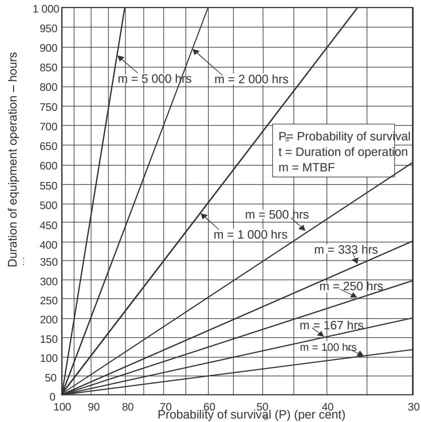
Figure F-1. Plot of P_s = 100 e^{-t/m}
